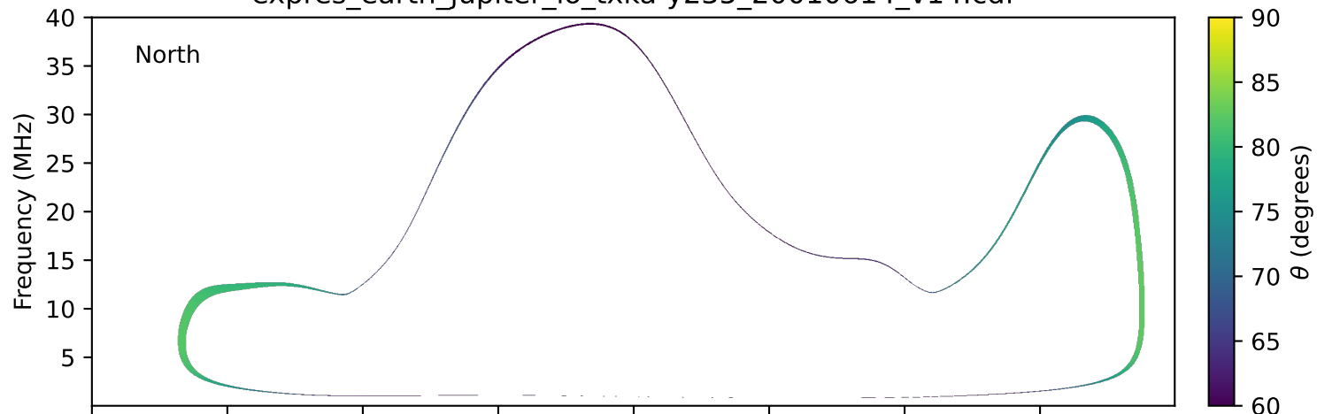
expres_earth_jupiter_io_txka-y235_20010614_v14.cdf
