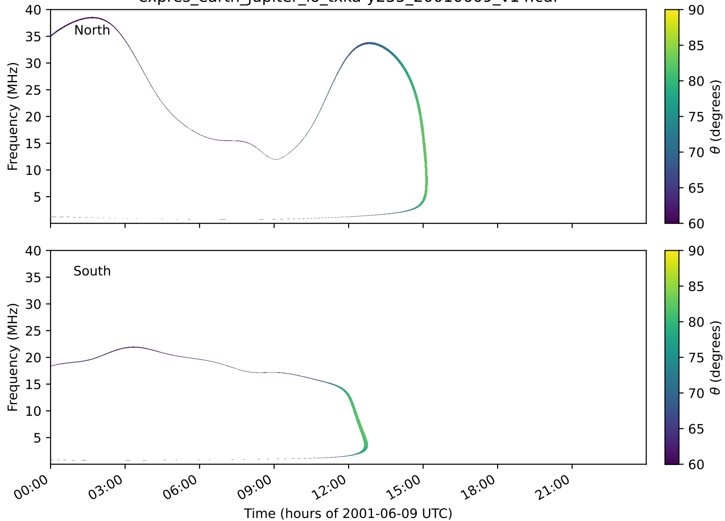
expres_earth_jupiter_io_txka-y235_20010609_v14.cdf
