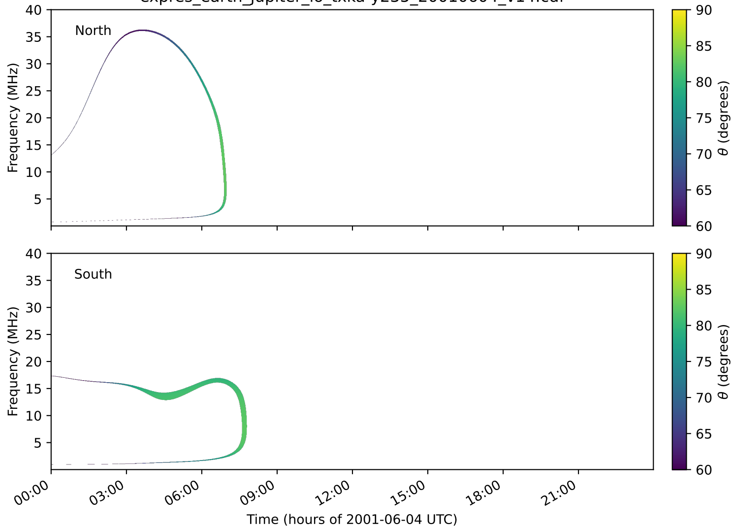
expres_earth_jupiter_io_txka-y235_20010604_v14.cdf
