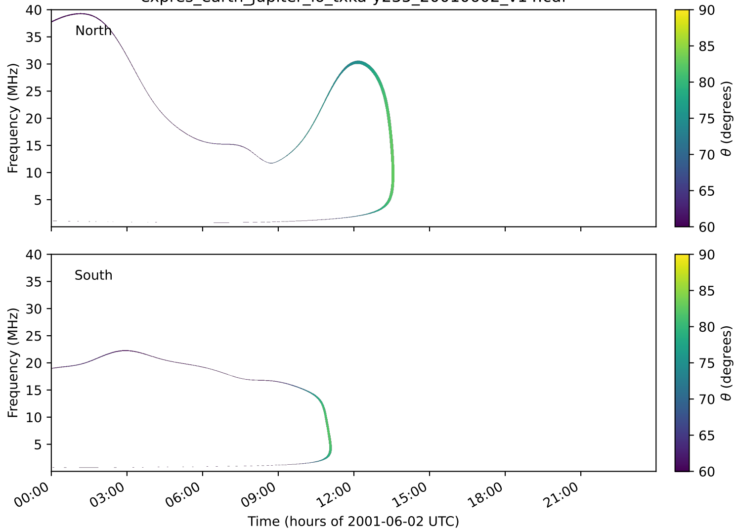
expres_earth_jupiter_io_txka-y235_20010602_v14.cdf
