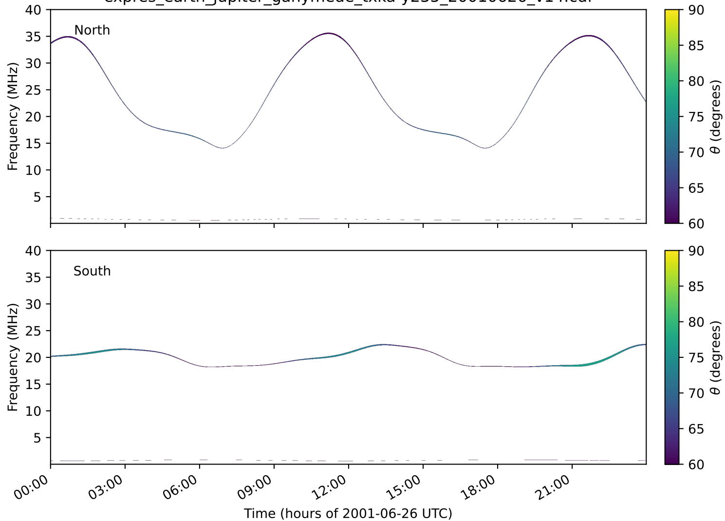
expres_earth_jupiter_ganymede_txka-y235_20010626_v14.cdf
