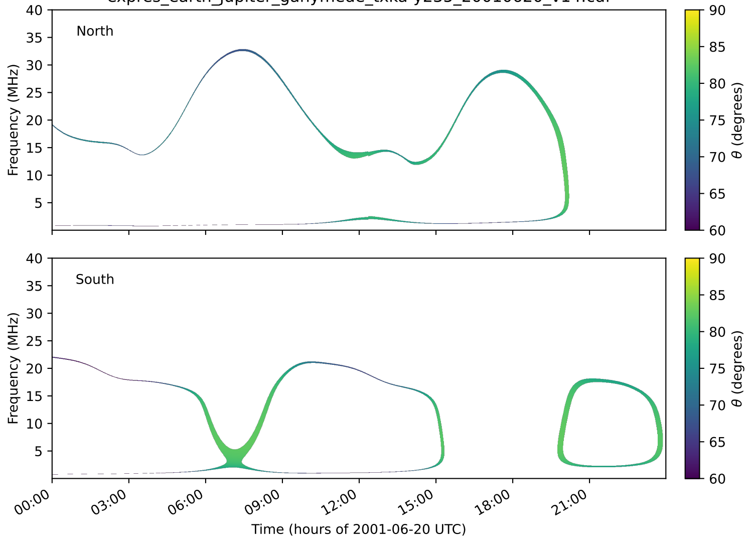
expres_earth_jupiter_ganymede_txka-y235_20010620_v14.cdf
