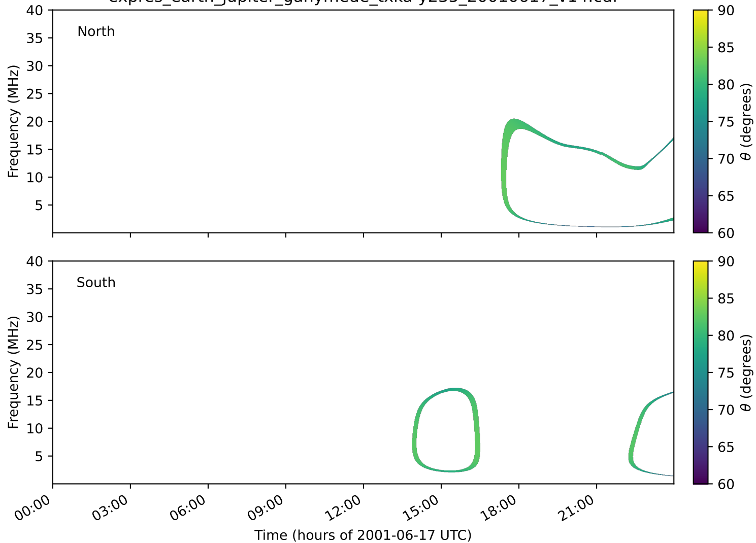
expres_earth_jupiter_ganymede_txka-y235_20010617_v14.cdf
