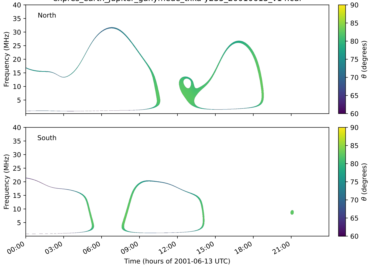
expres_earth_jupiter_ganymede_txka-y235_20010613_v14.cdf
