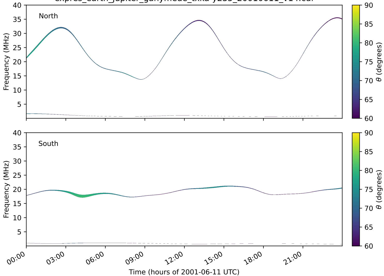
expres_earth_jupiter_ganymede_txka-y235_20010611_v14.cdf
