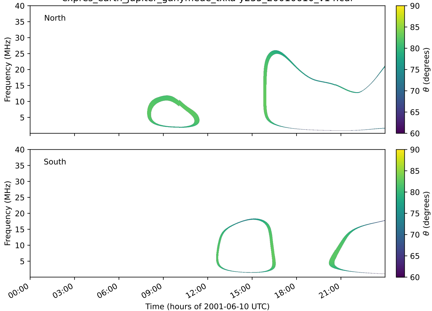
expres_earth_jupiter_ganymede_txka-y235_20010610_v14.cdf
