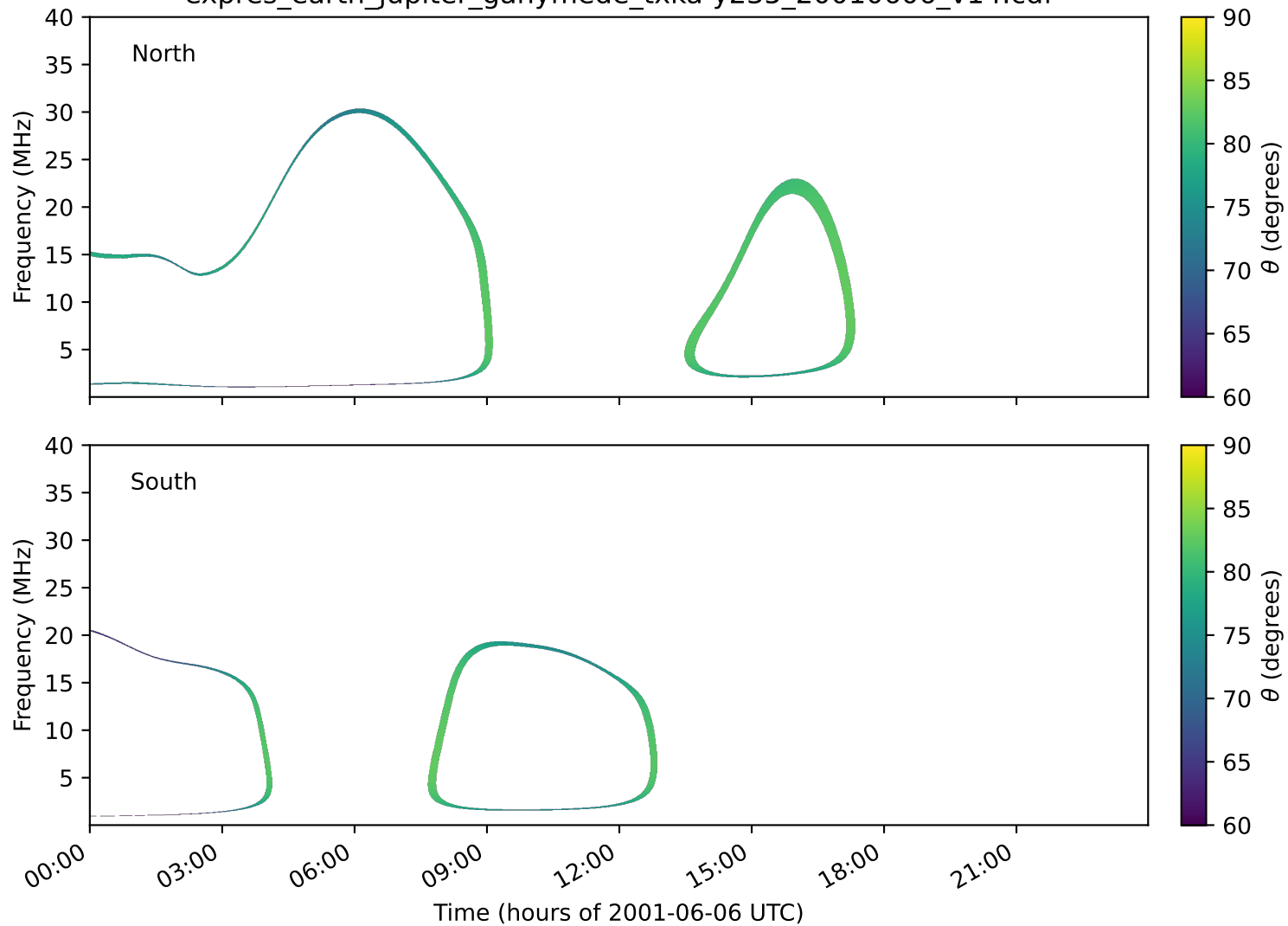
expres_earth_jupiter_ganymede_txka-y235_20010606_v14.cdf
