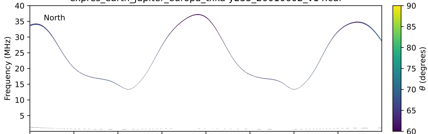
expres_earth_jupiter_europa_txka-y235_20010602_v14.cdf
