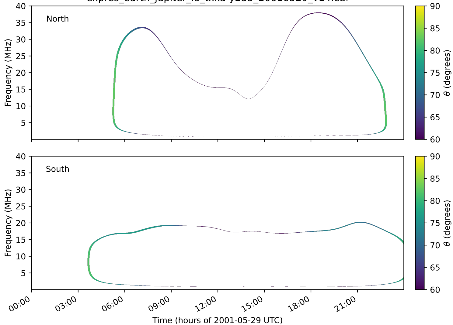
expres_earth_jupiter_io_txka-y235_20010529_v14.cdf
