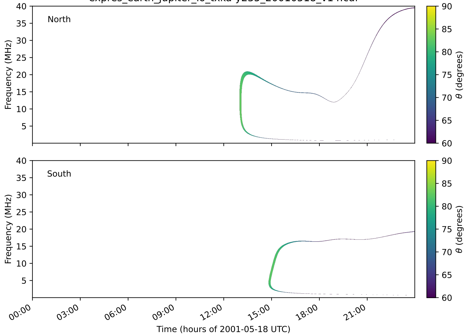
expres_earth_jupiter_io_txka-y235_20010518_v14.cdf
