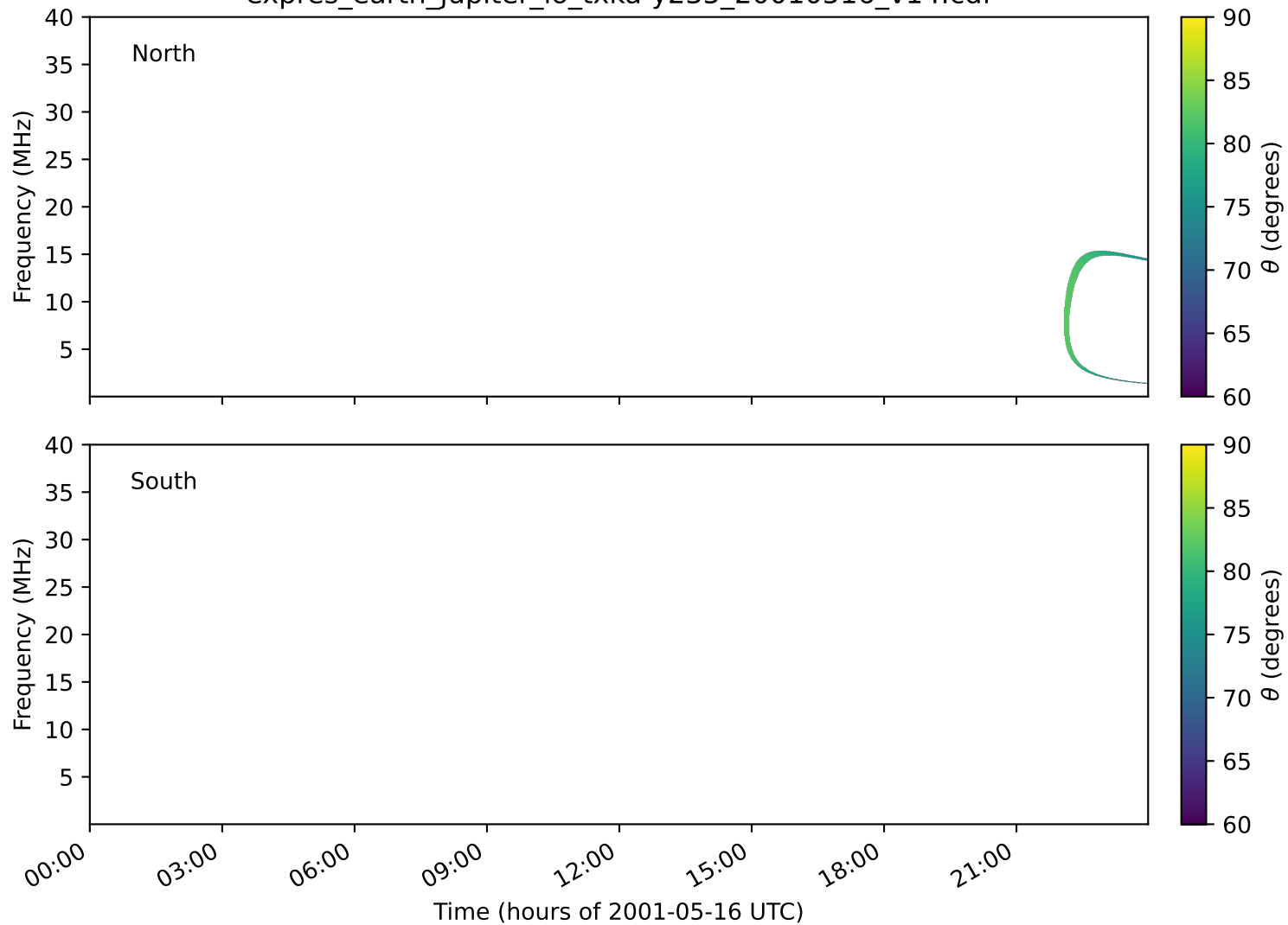
expres_earth_jupiter_io_txka-y235_20010516_v14.cdf
