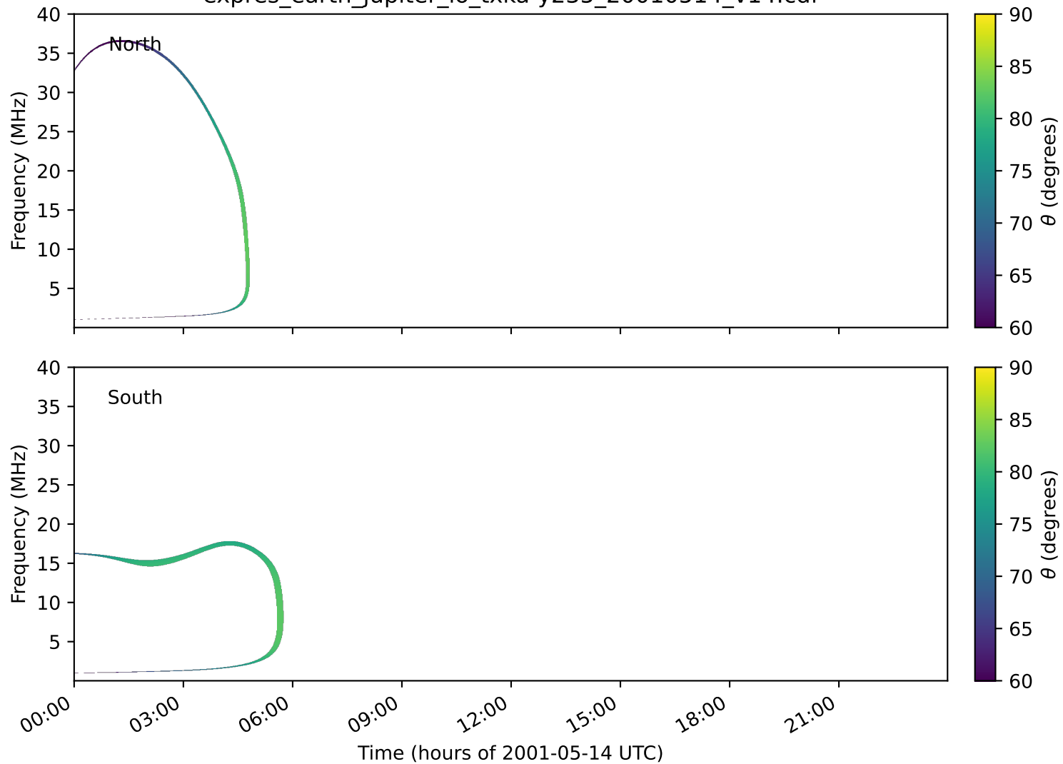
expres_earth_jupiter_io_txka-y235_20010514_v14.cdf
