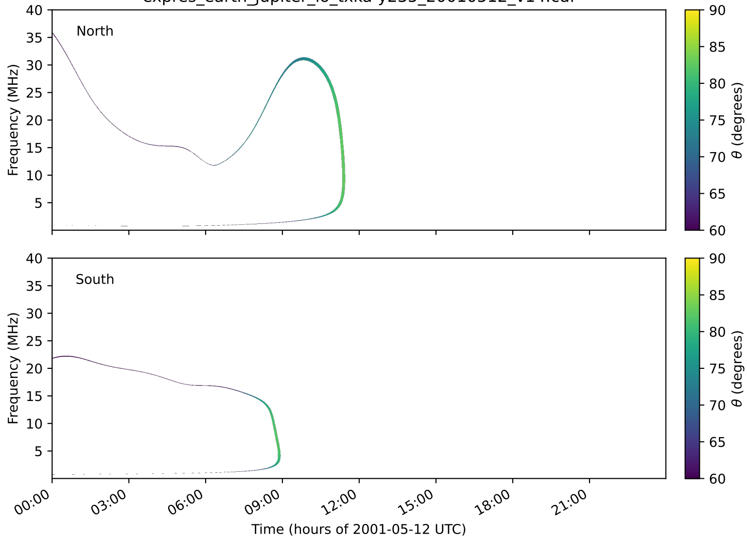
expres_earth_jupiter_io_txka-y235_20010512_v14.cdf
