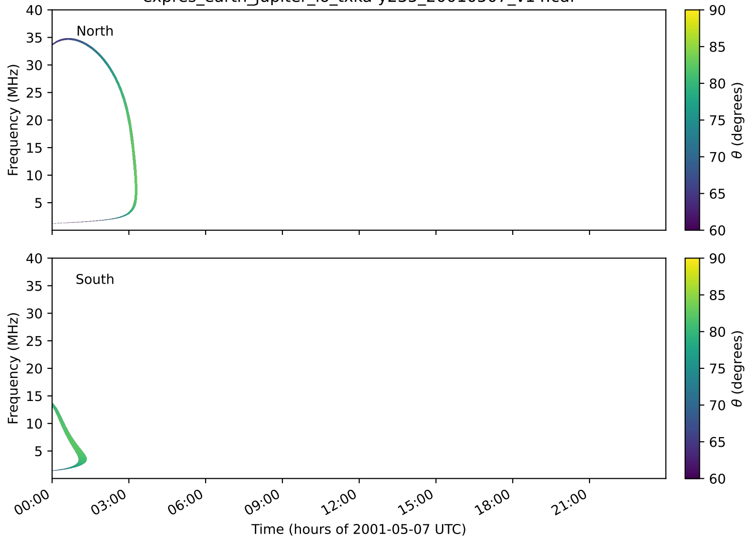
expres_earth_jupiter_io_txka-y235_20010507_v14.cdf
