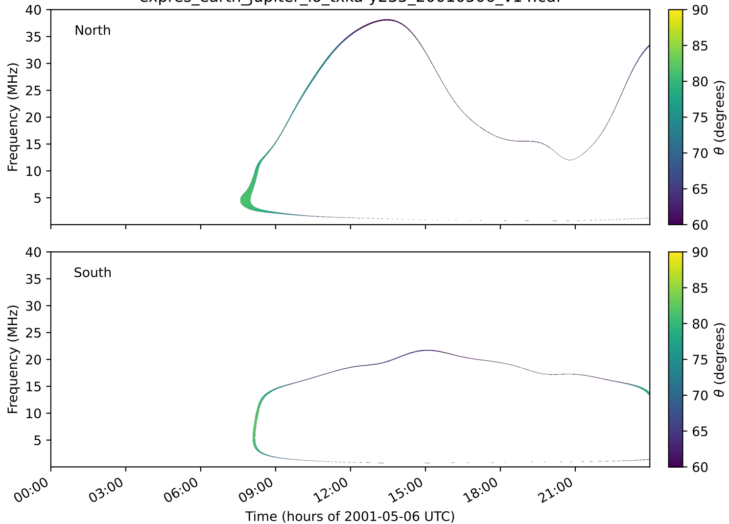
expres_earth_jupiter_io_txka-y235_20010506_v14.cdf
