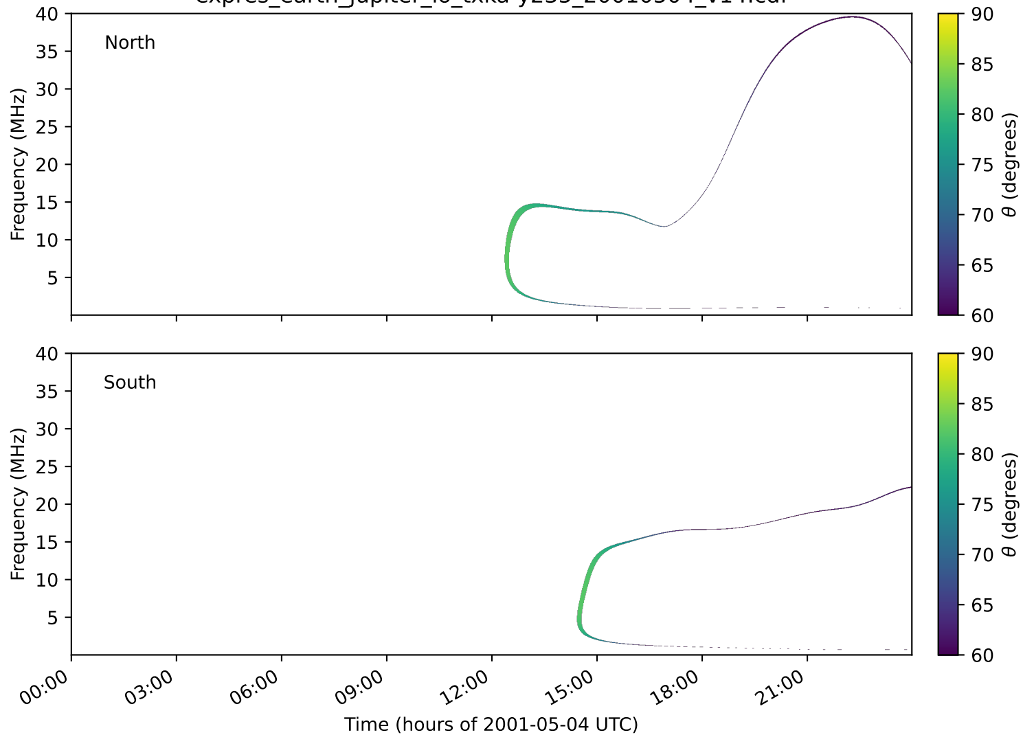
expres_earth_jupiter_io_txka-y235_20010504_v14.cdf
