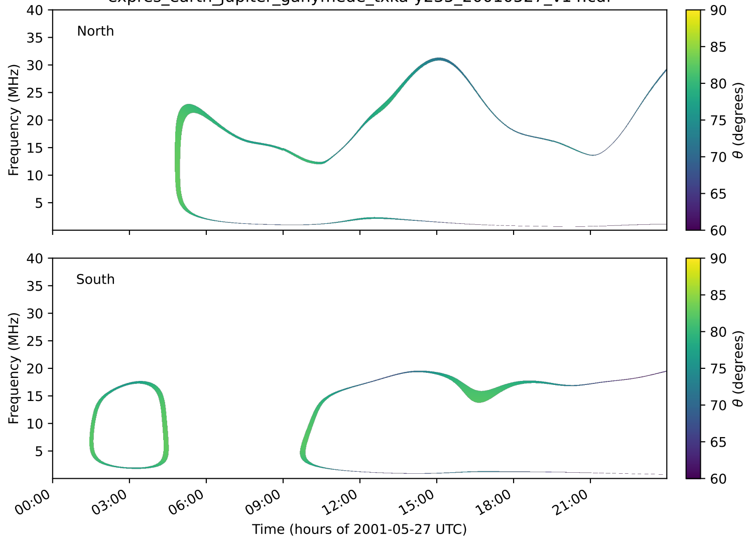
expres_earth_jupiter_ganymede_txka-y235_20010527_v14.cdf
