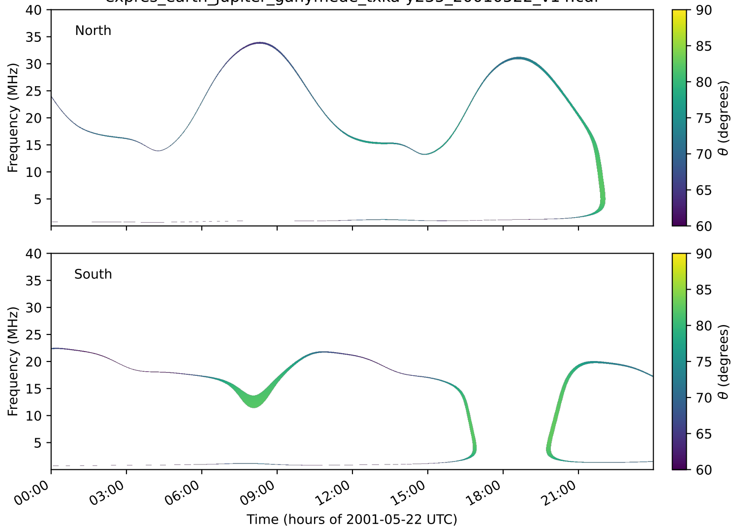
expres_earth_jupiter_ganymede_txka-y235_20010522_v14.cdf
