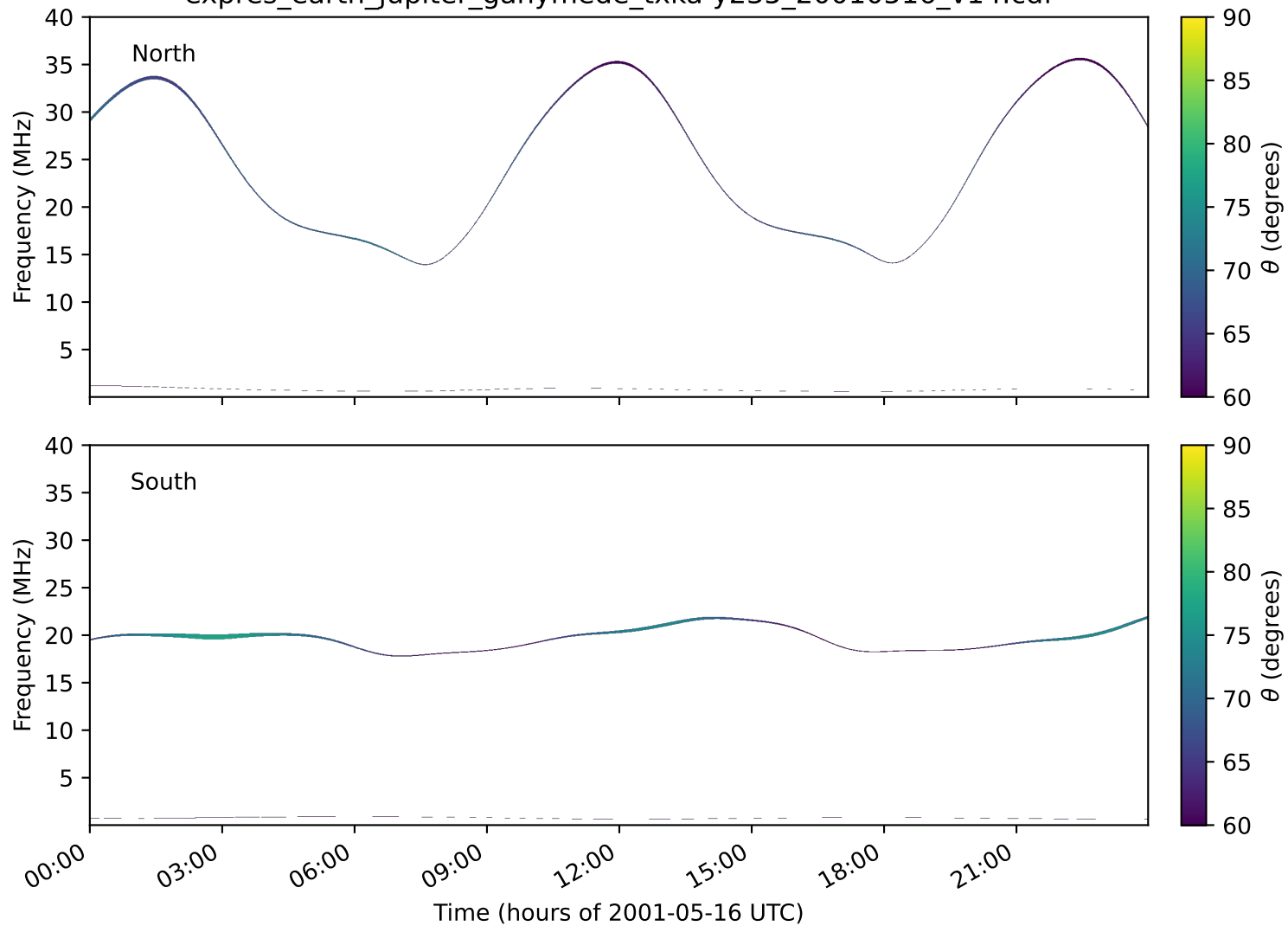
expres_earth_jupiter_ganymede_txka-y235_20010516_v14.cdf
