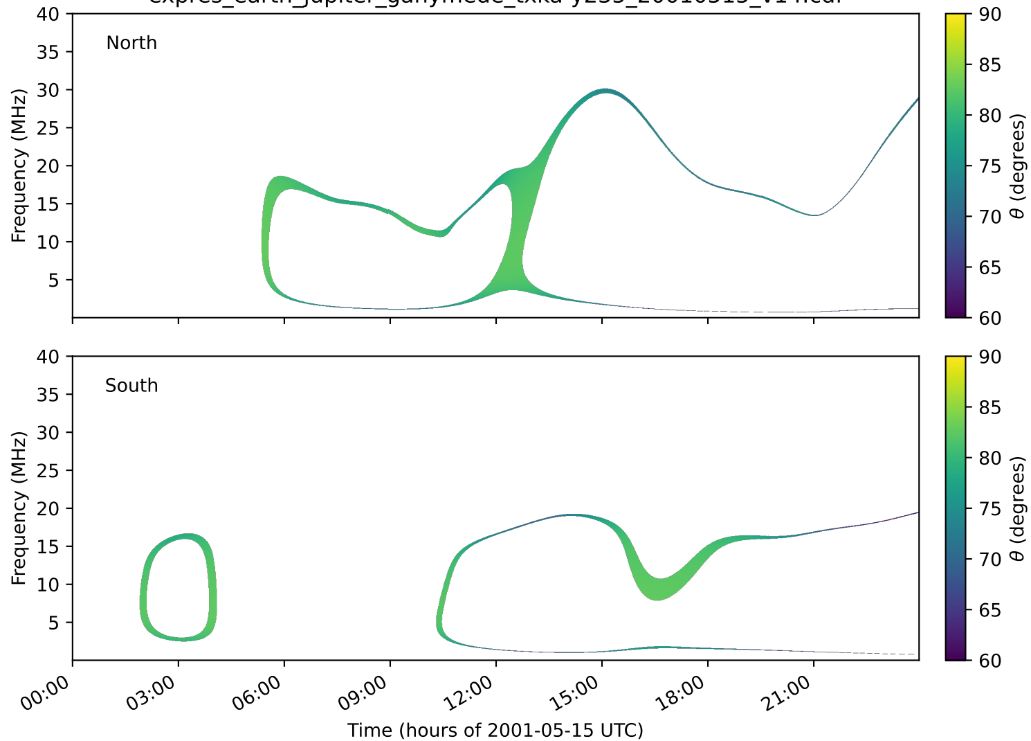
expres_earth_jupiter_ganymede_txka-y235_20010515_v14.cdf
