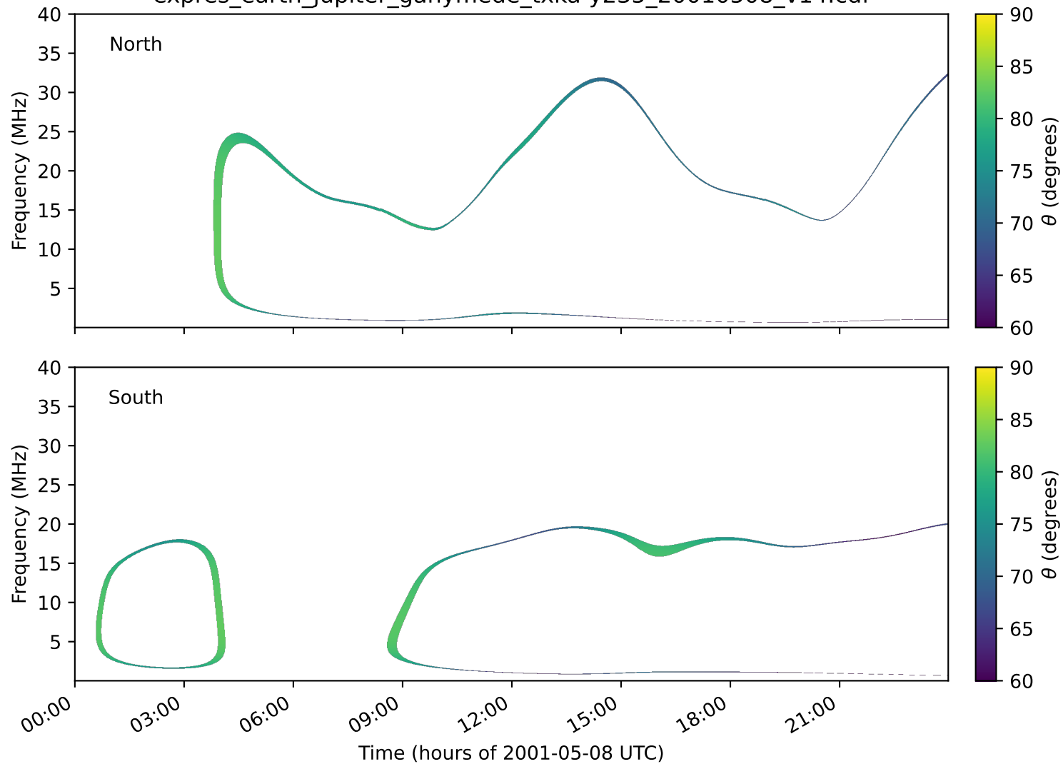
expres_earth_jupiter_ganymede_txka-y235_20010508_v14.cdf
