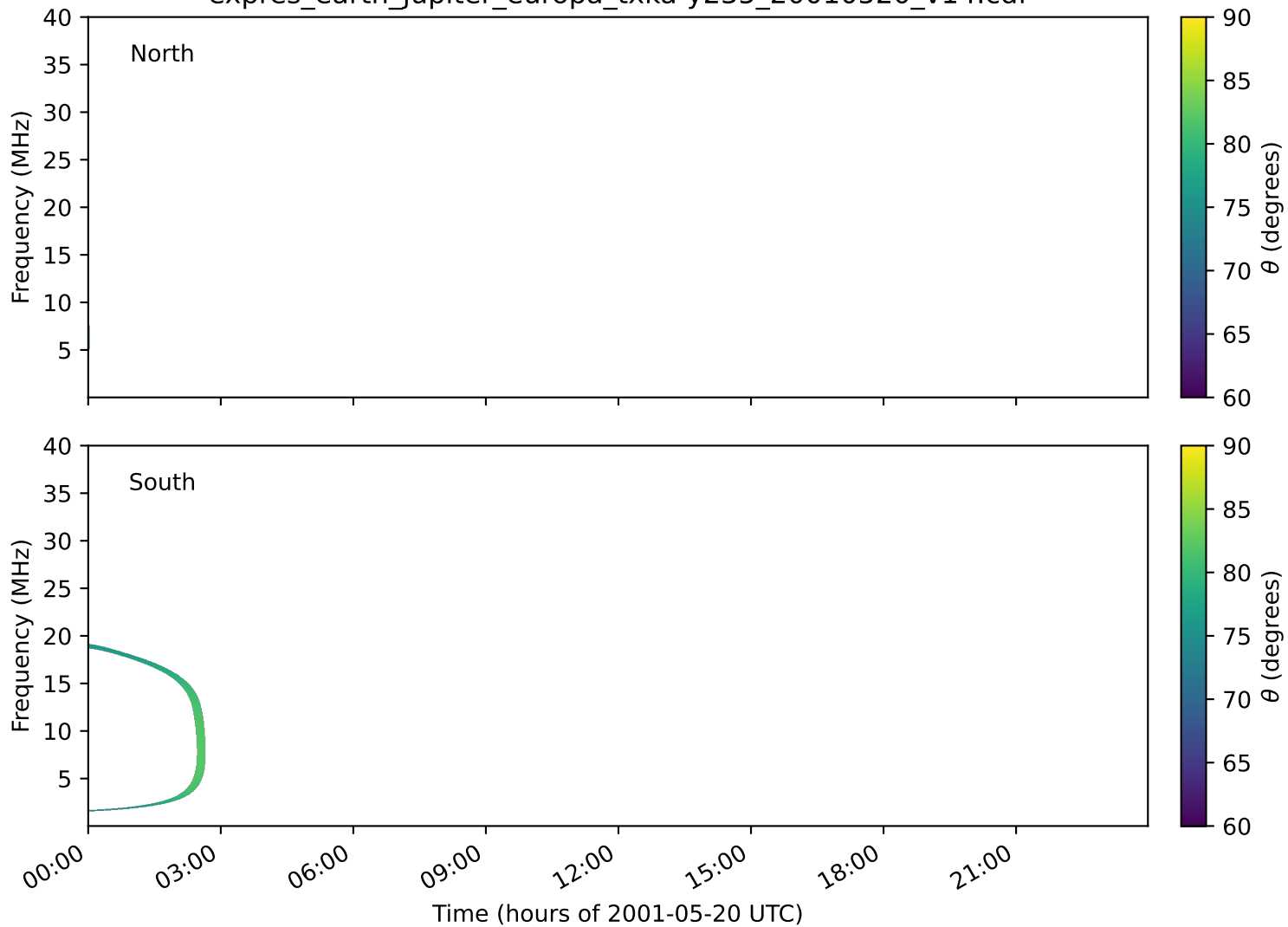
expres_earth_jupiter_europa_txka-y235_20010520_v14.cdf
