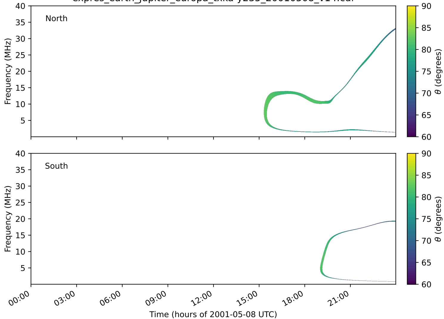
expres_earth_jupiter_europa_txka-y235_20010508_v14.cdf
