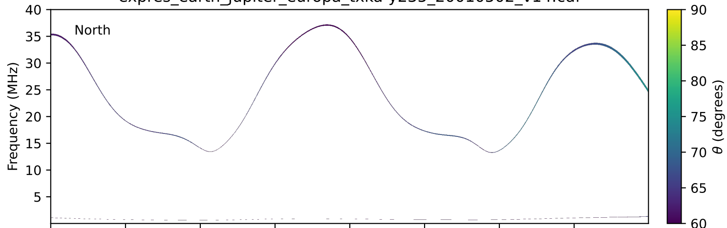
expres_earth_jupiter_europa_txka-y235_20010502_v14.cdf
