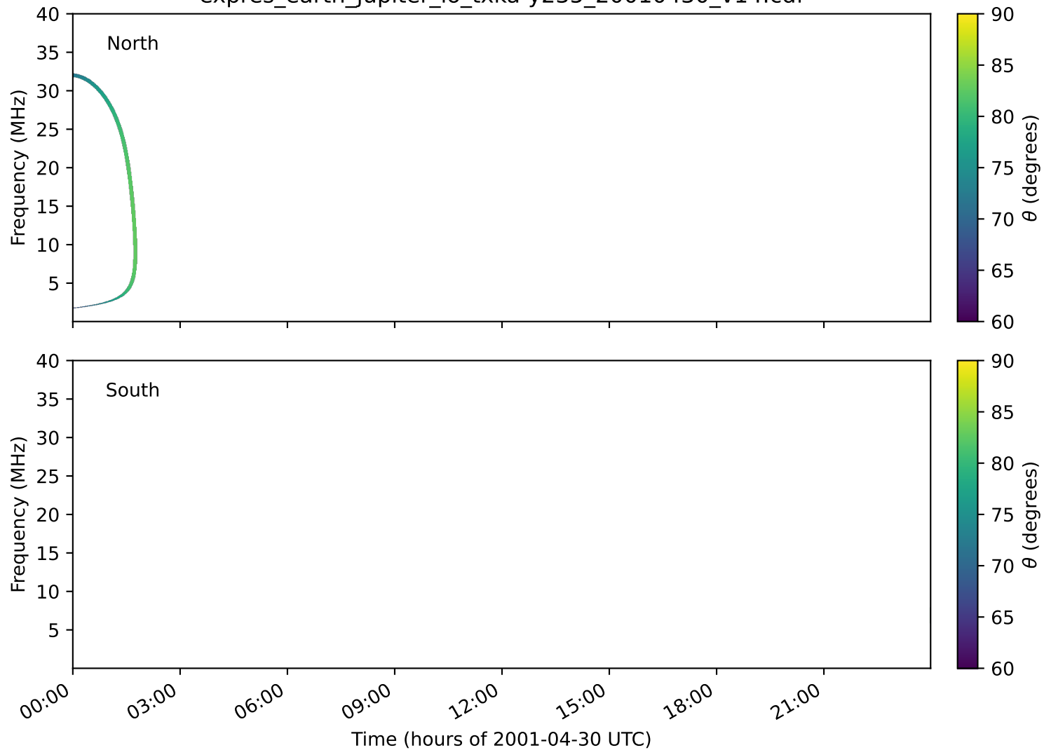
expres_earth_jupiter_io_txka-y235_20010430_v14.cdf
