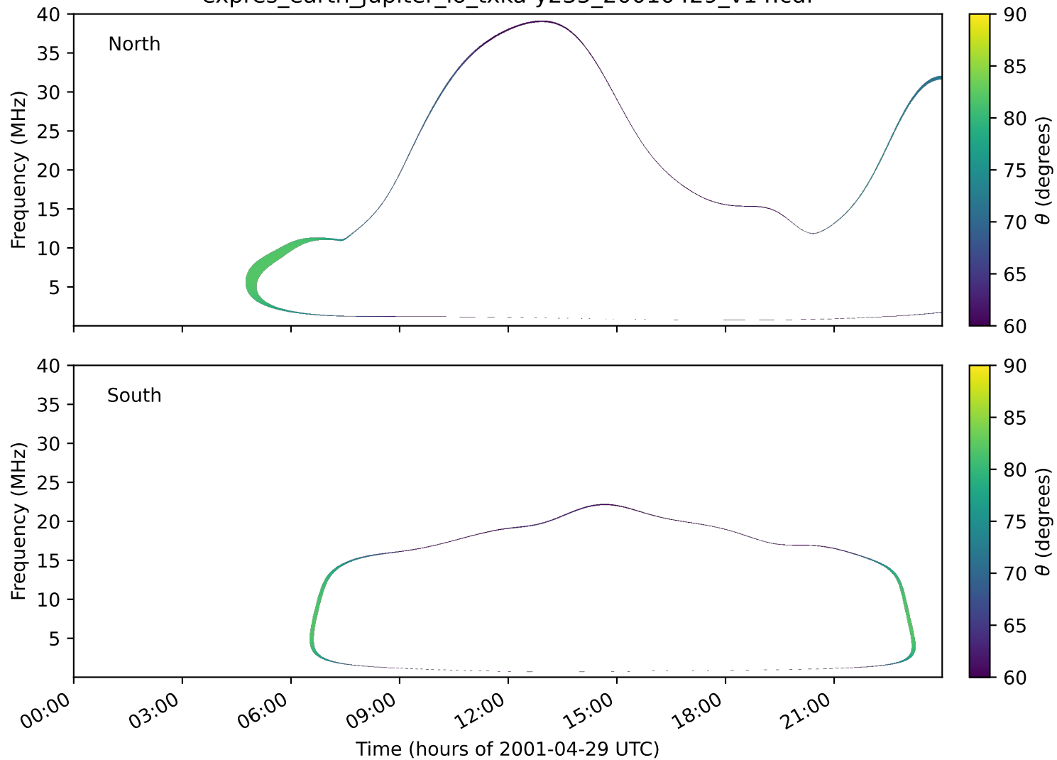
expres_earth_jupiter_io_txka-y235_20010429_v14.cdf
