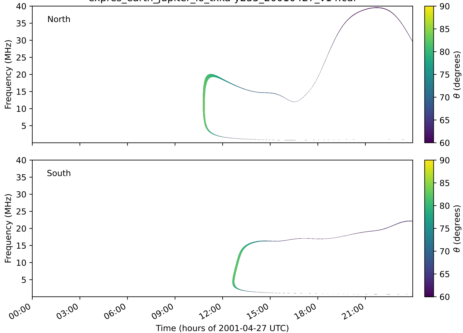
expres_earth_jupiter_io_txka-y235_20010427_v14.cdf
