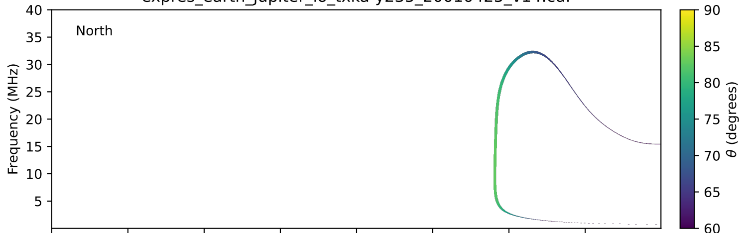
expres_earth_jupiter_io_txka-y235_20010425_v14.cdf
