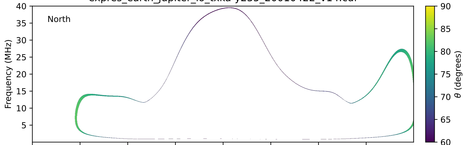
expres_earth_jupiter_io_txka-y235_20010422_v14.cdf
