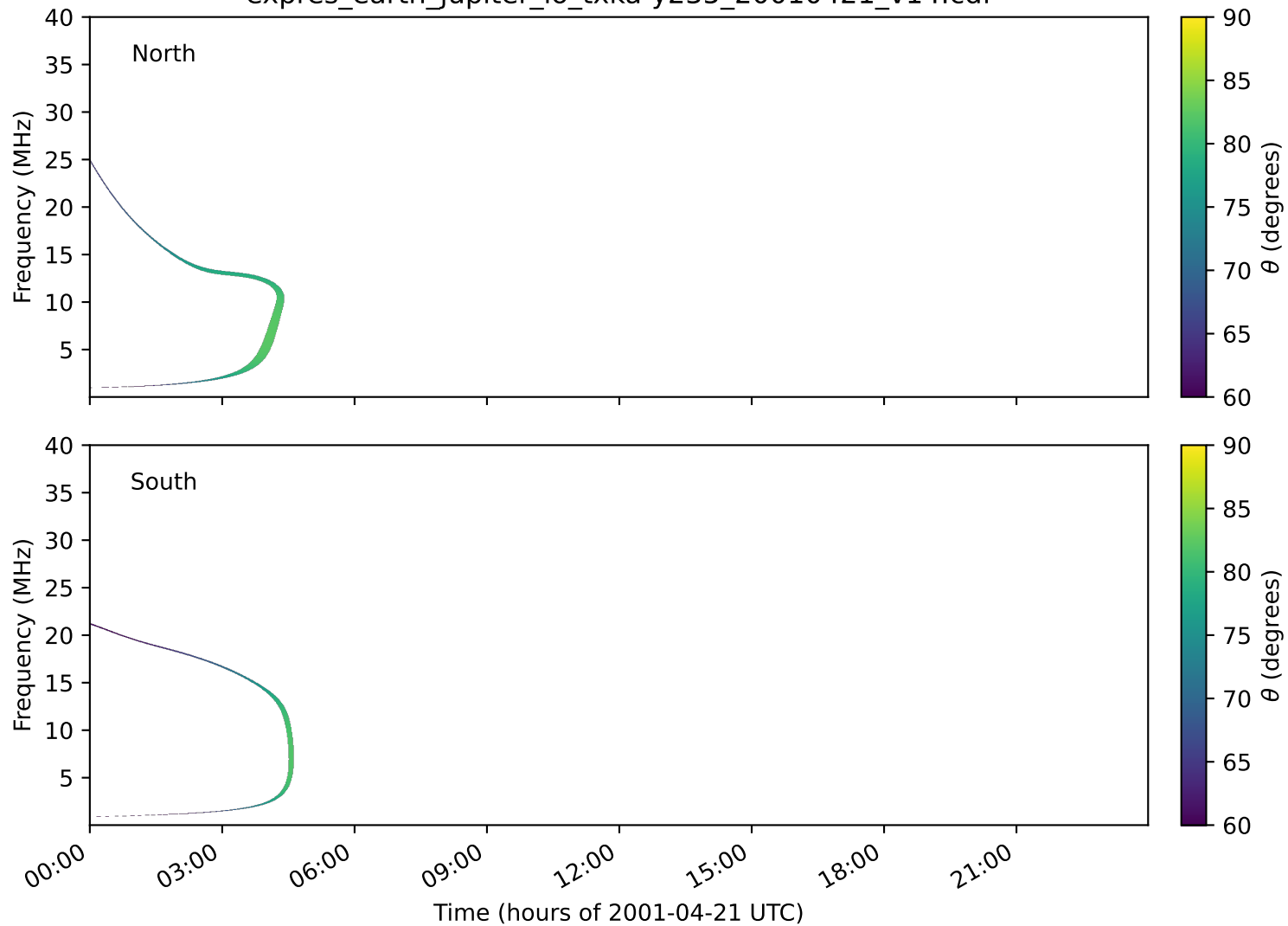
expres_earth_jupiter_io_txka-y235_20010421_v14.cdf
