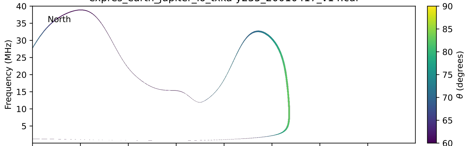
expres_earth_jupiter_io_txka-y235_20010417_v14.cdf
