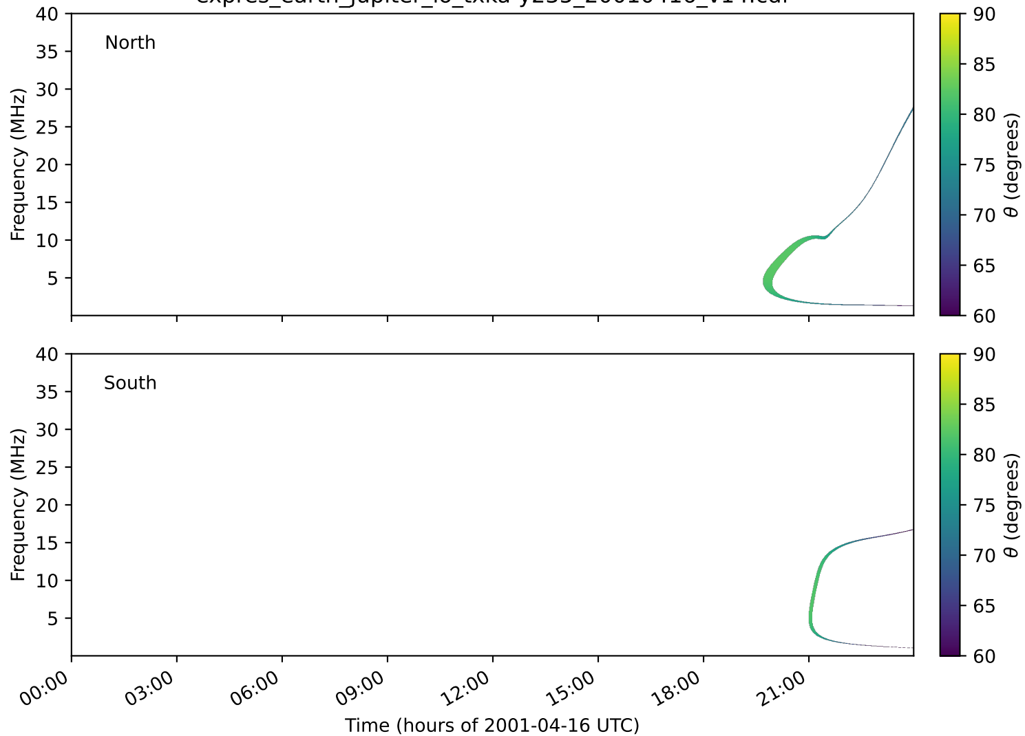
expres_earth_jupiter_io_txka-y235_20010416_v14.cdf
