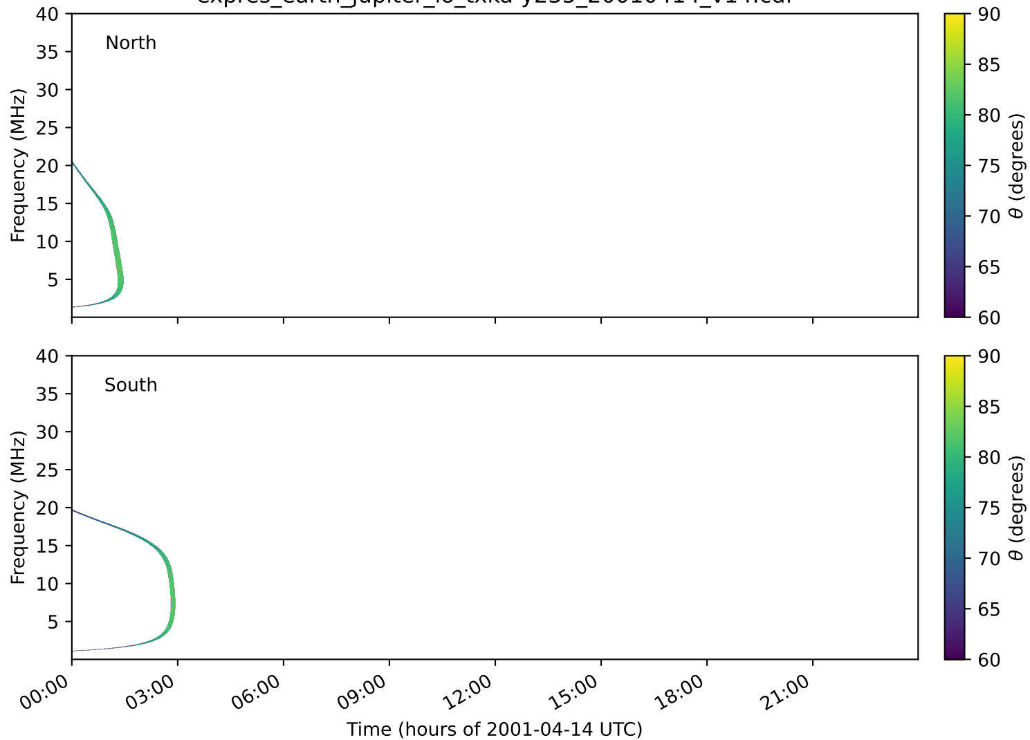
expres_earth_jupiter_io_txka-y235_20010414_v14.cdf
