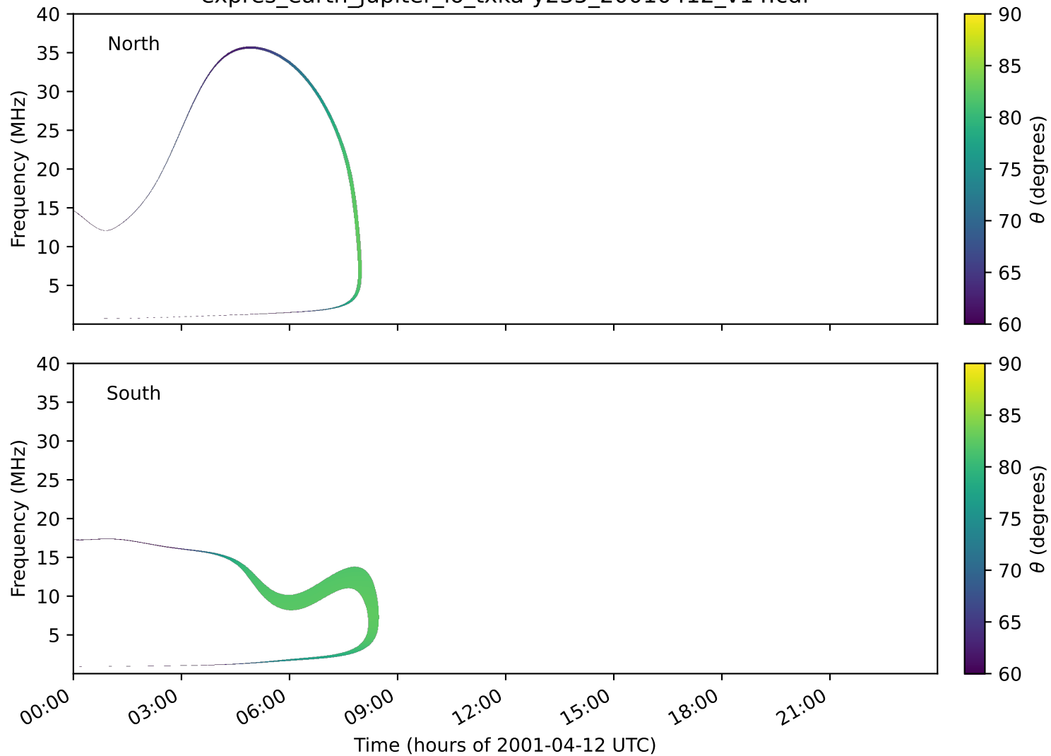
expres_earth_jupiter_io_txka-y235_20010412_v14.cdf
