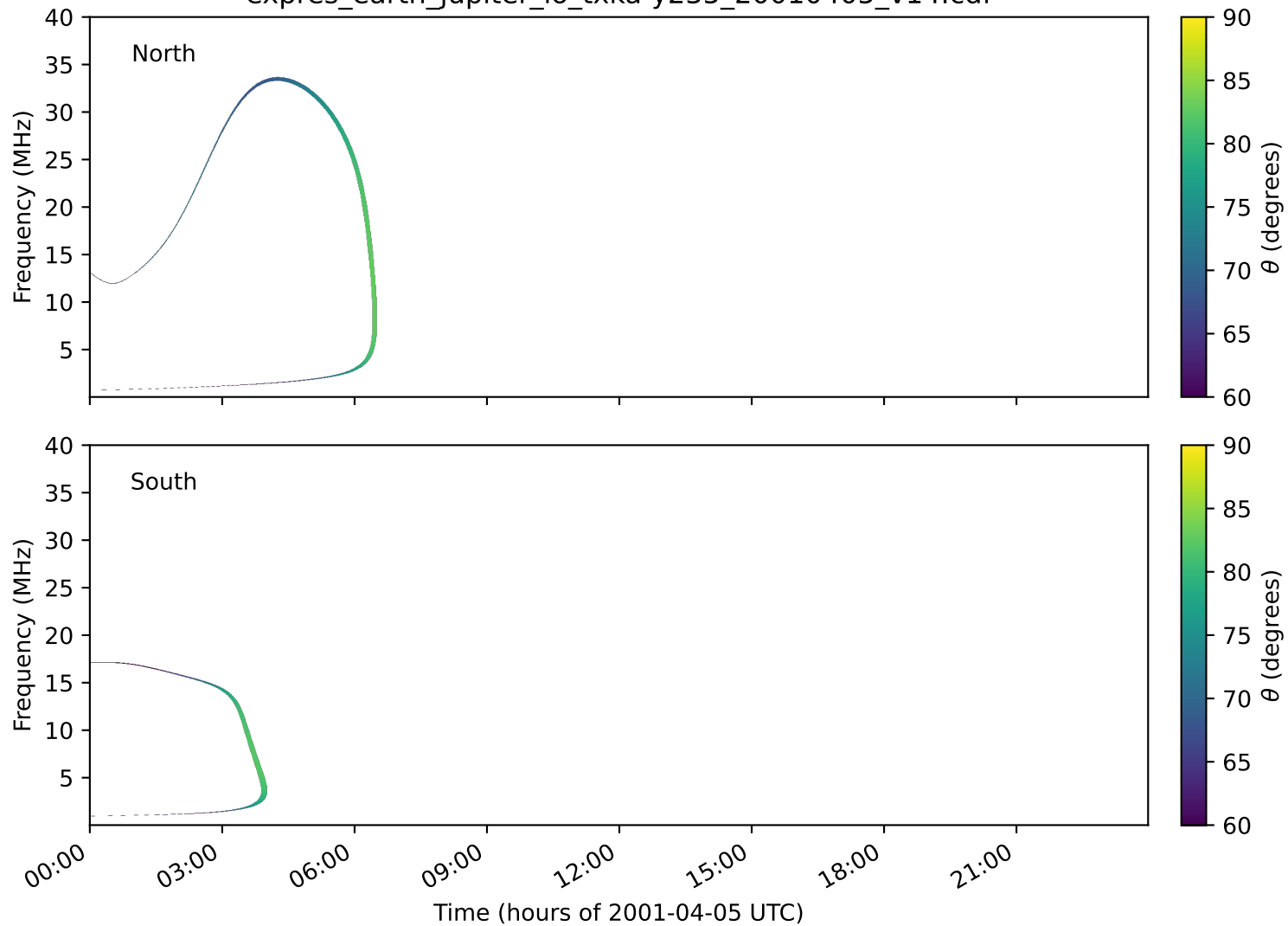
expres_earth_jupiter_io_txka-y235_20010405_v14.cdf
