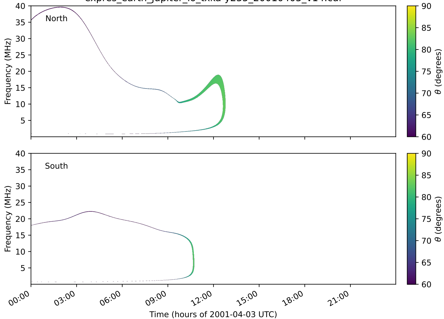
expres_earth_jupiter_io_txka-y235_20010403_v14.cdf
