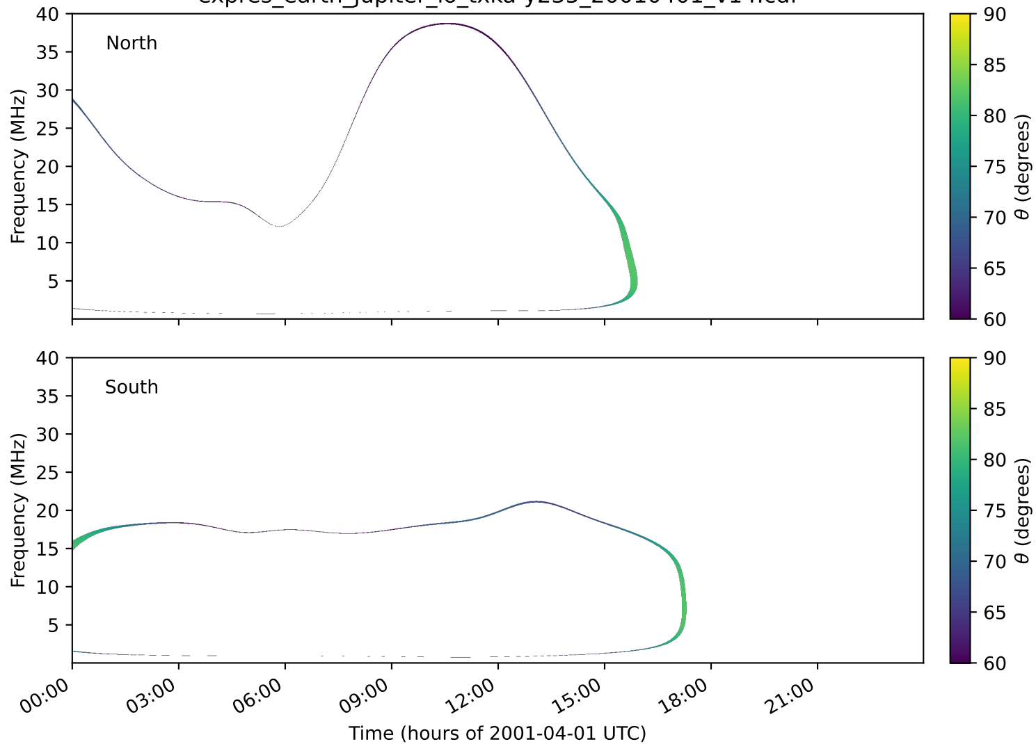
expres_earth_jupiter_io_txka-y235_20010401_v14.cdf
