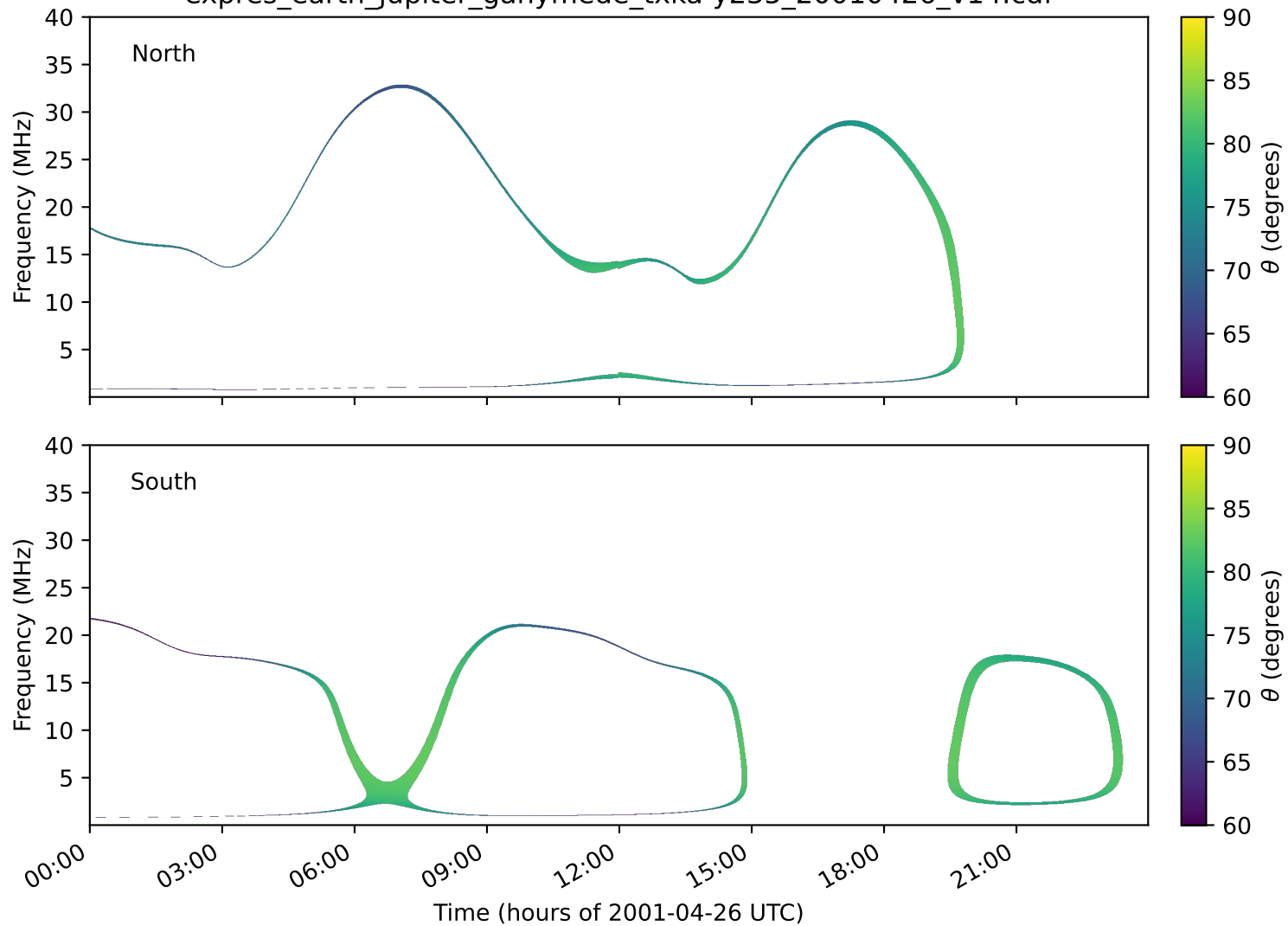
expres_earth_jupiter_ganymede_txka-y235_20010426_v14.cdf
