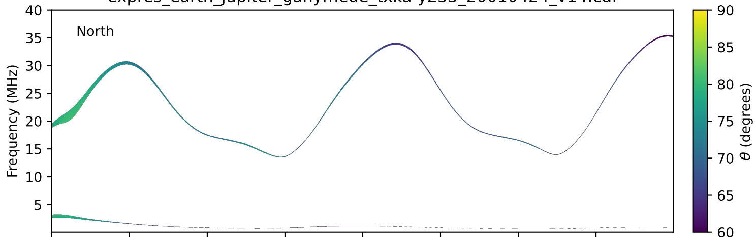
expres_earth_jupiter_ganymede_txka-y235_20010424_v14.cdf
