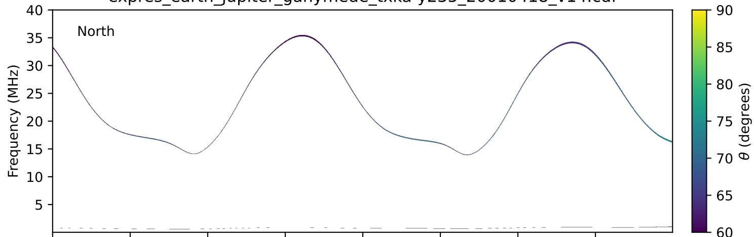
expres_earth_jupiter_ganymede_txka-y235_20010418_v14.cdf
