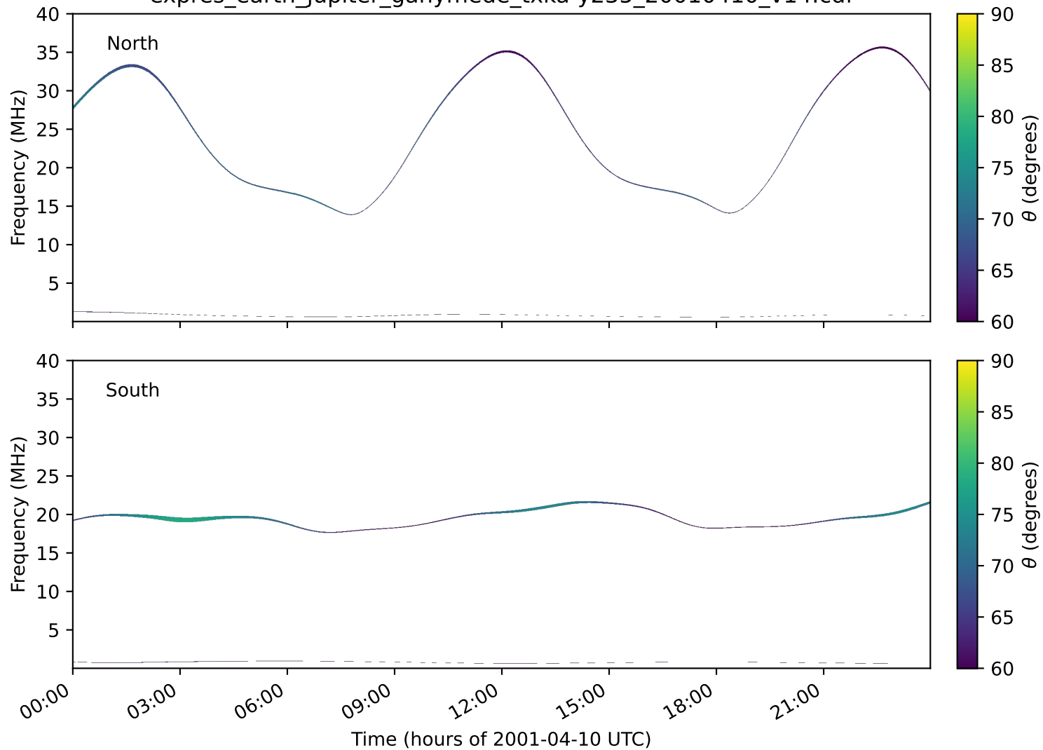
expres_earth_jupiter_ganymede_txka-y235_20010410_v14.cdf
