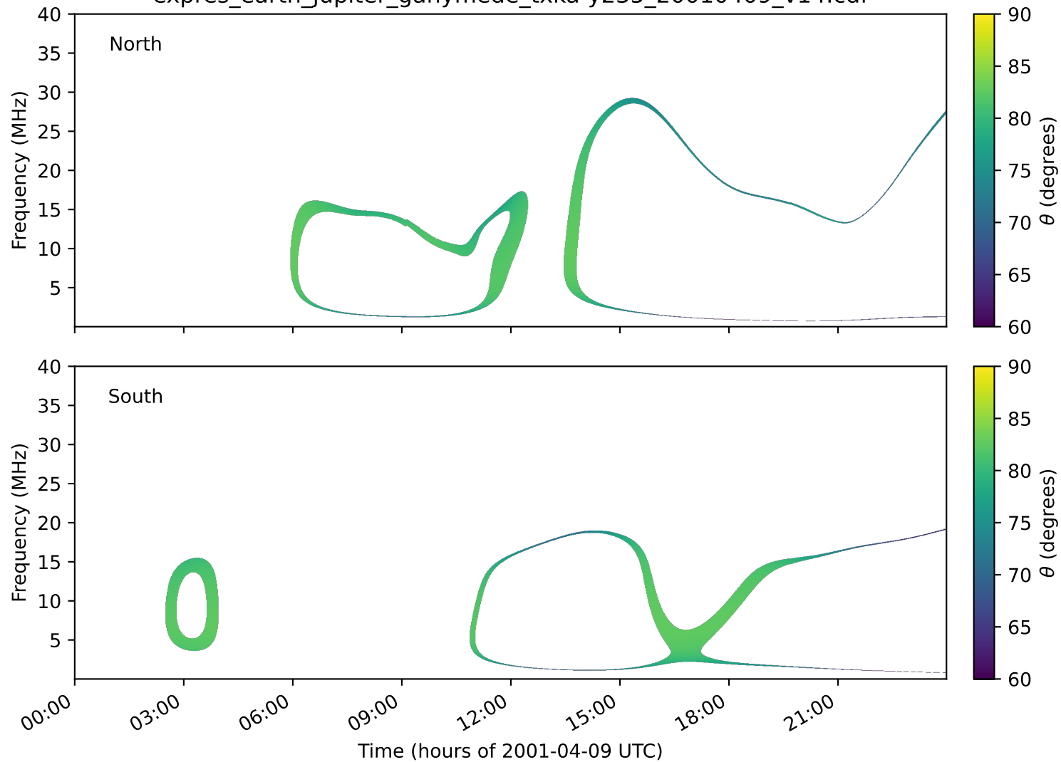
expres_earth_jupiter_ganymede_txka-y235_20010409_v14.cdf
