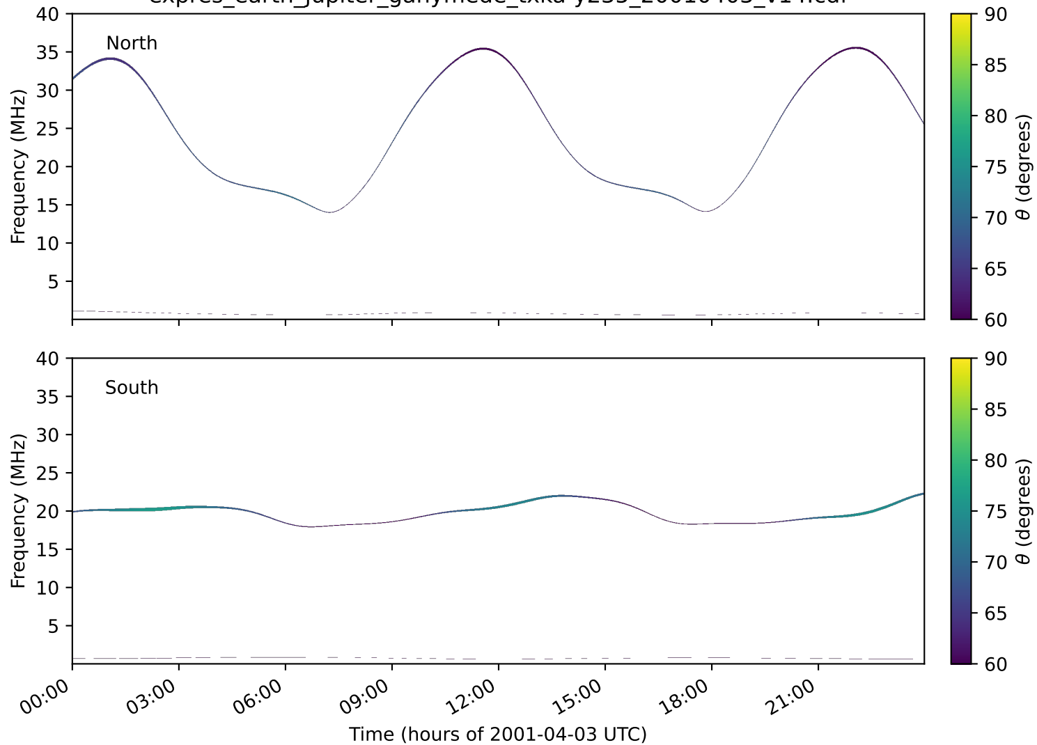
expres_earth_jupiter_ganymede_txka-y235_20010403_v14.cdf
