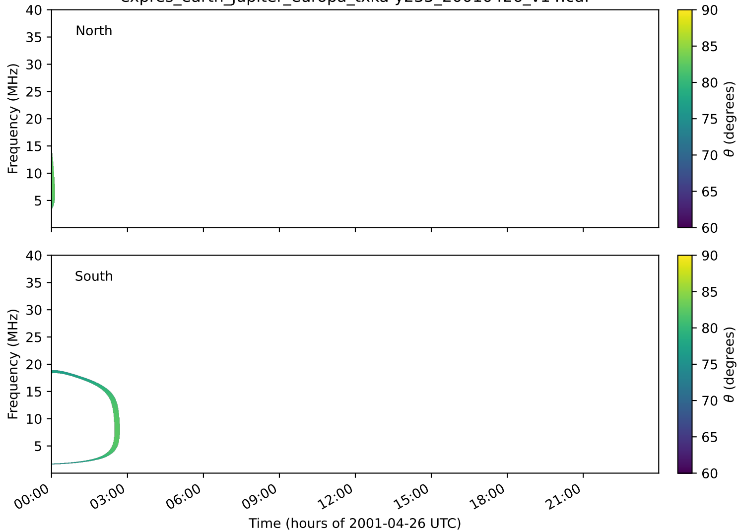
expres_earth_jupiter_europa_txka-y235_20010426_v14.cdf
