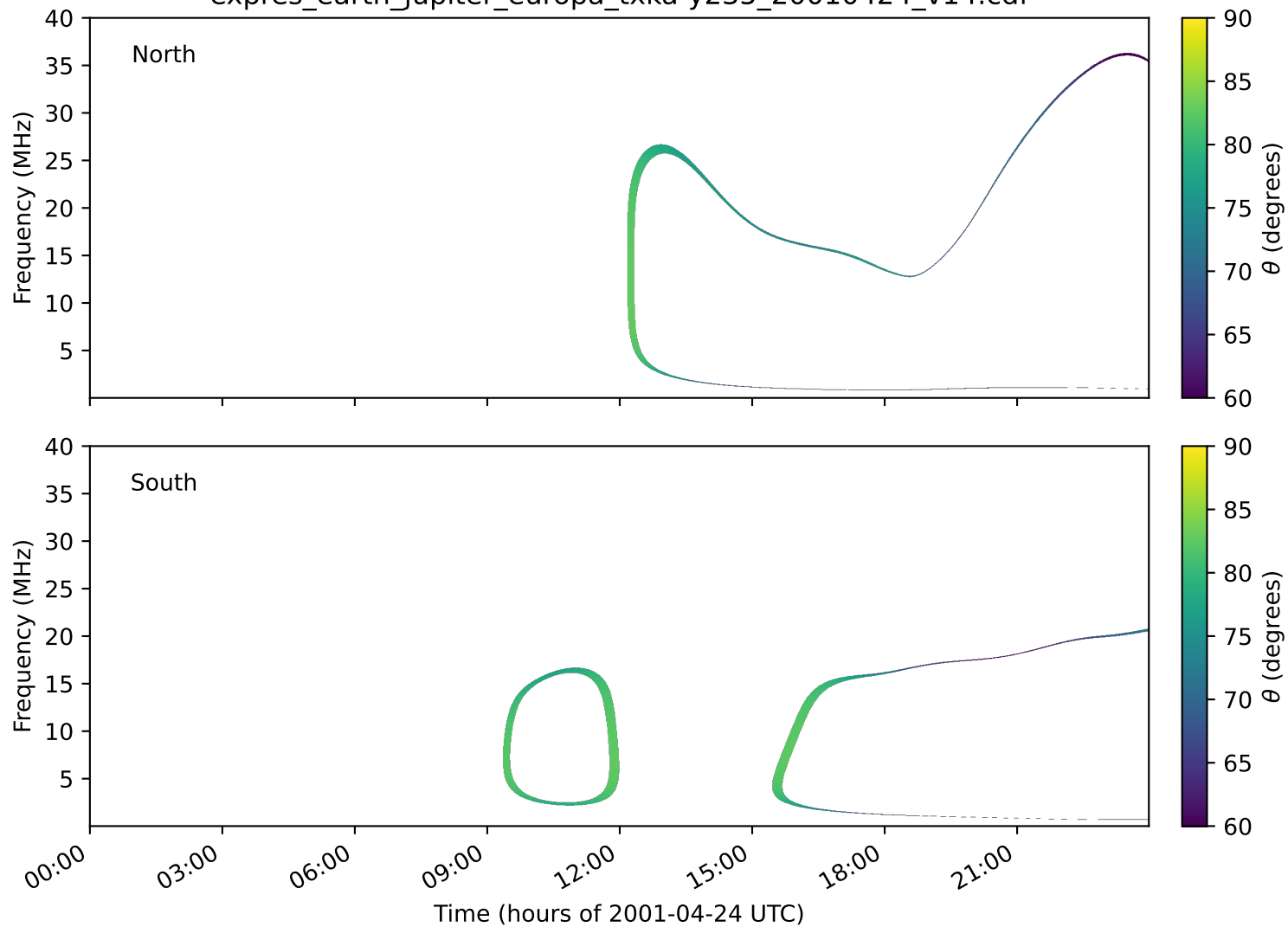
expres_earth_jupiter_europa_txka-y235_20010424_v14.cdf
