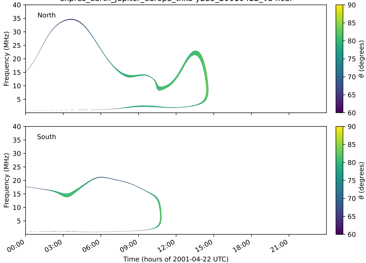
expres_earth_jupiter_europa_txka-y235_20010422_v14.cdf
